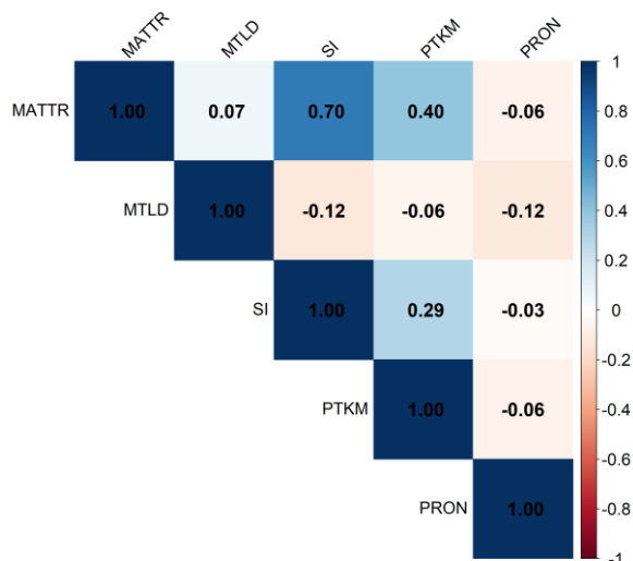
Figure 1: Correlation Heatmap
