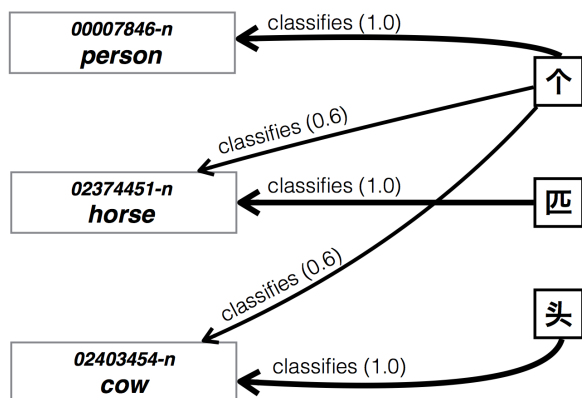
Figure 1: Example of classifier network
