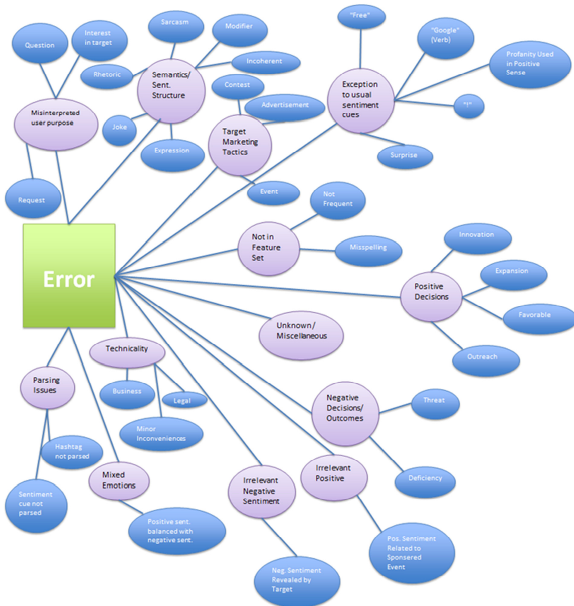
Figure 1: Twitter Sentiment Error Analysis Taxonomy
