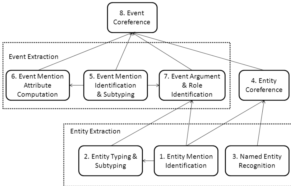
Figure 1: The architecture of SinoCoreferencer.
