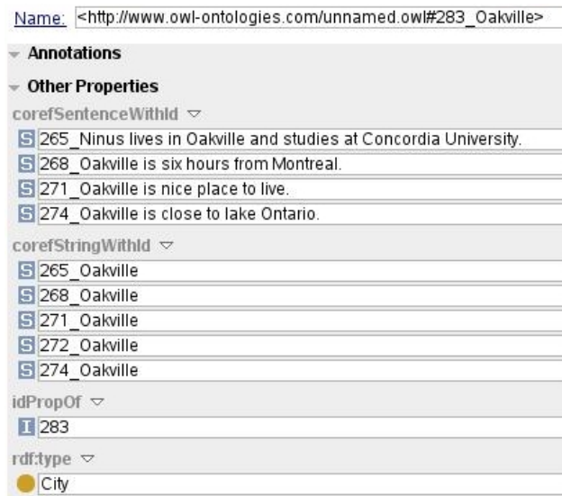
Figure 7: Coreference Chain Relationships exported into an OWL Ontology
