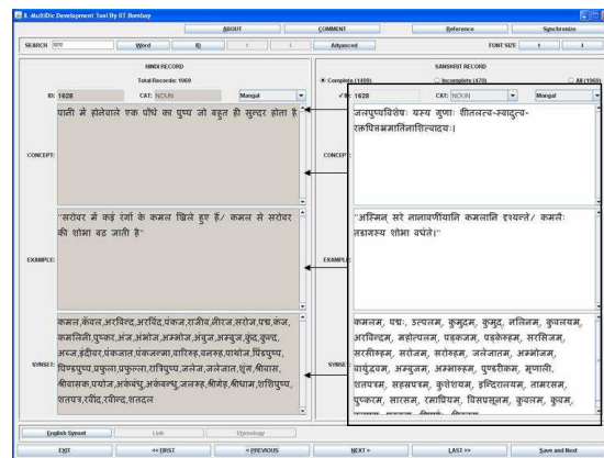
Figure 5: Lexicographer’s interface.
