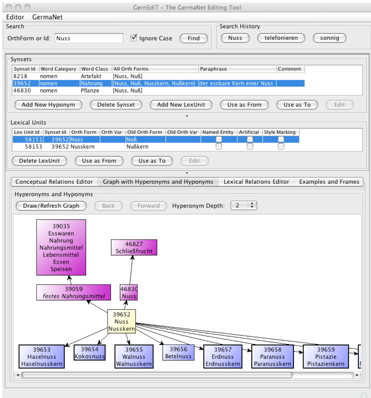
Figure 2: Main view of GernEdiT
