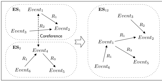
Figure 2: Unifying event structures.
