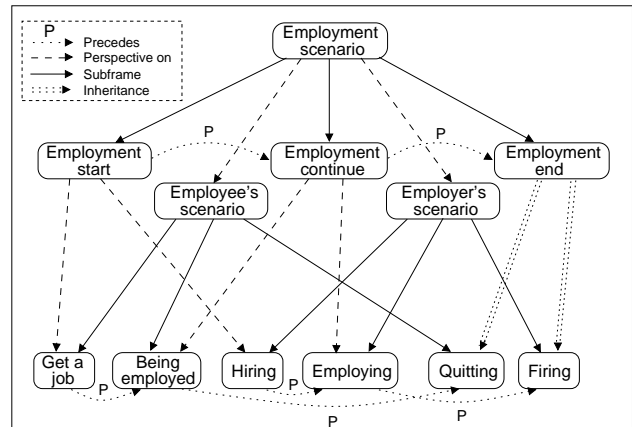
Figure 1: Building FrameNet scenarios using frame relations.
