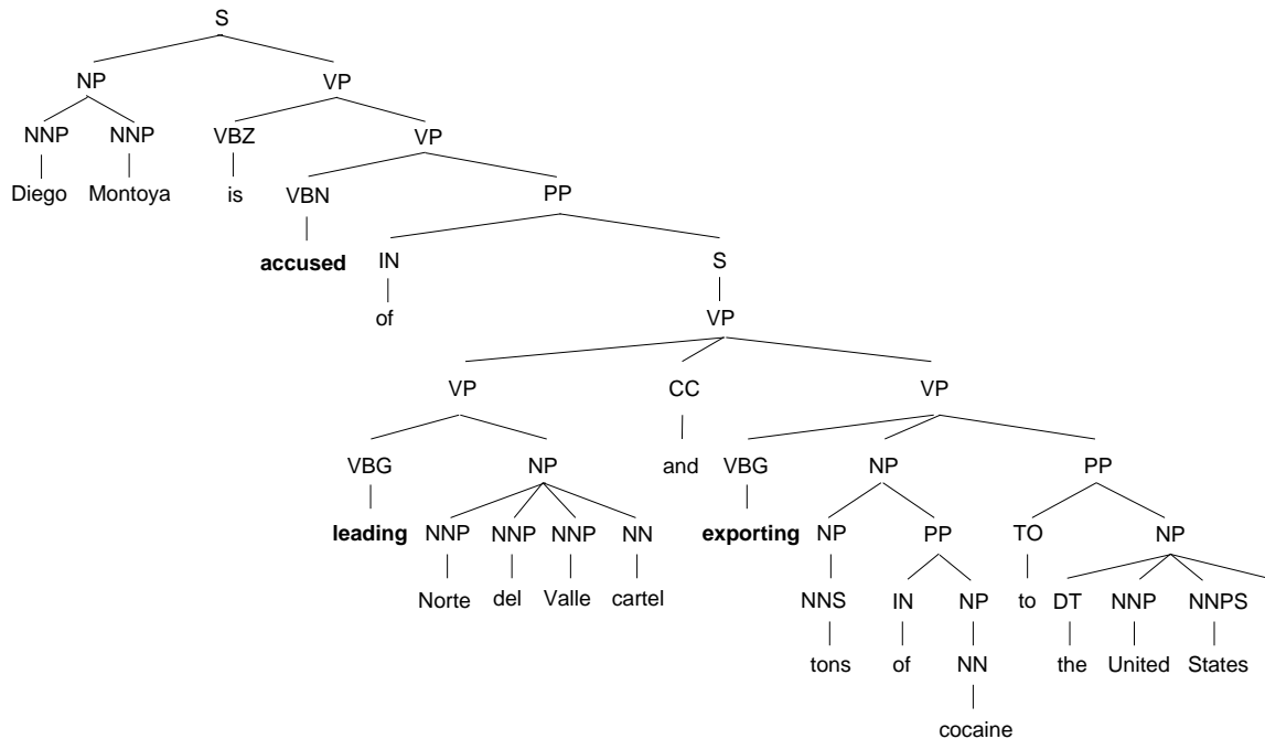
Figure 4: Syntactic parse tree representation of the sentence S_1 .
