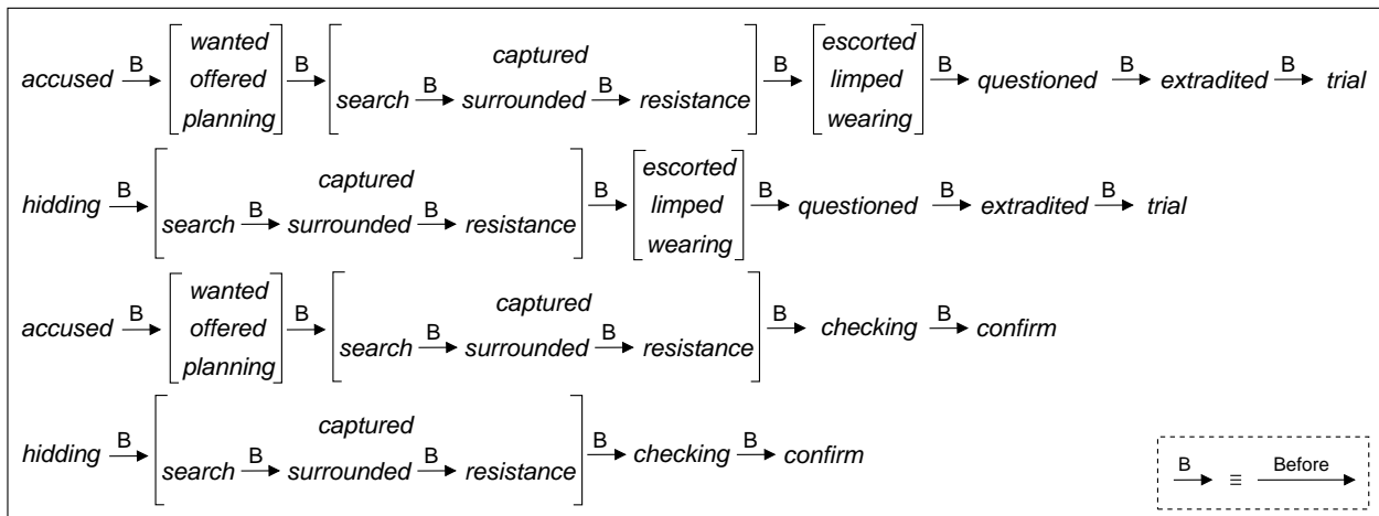
Figure 7: Deriving chronologies of events from event structures.
