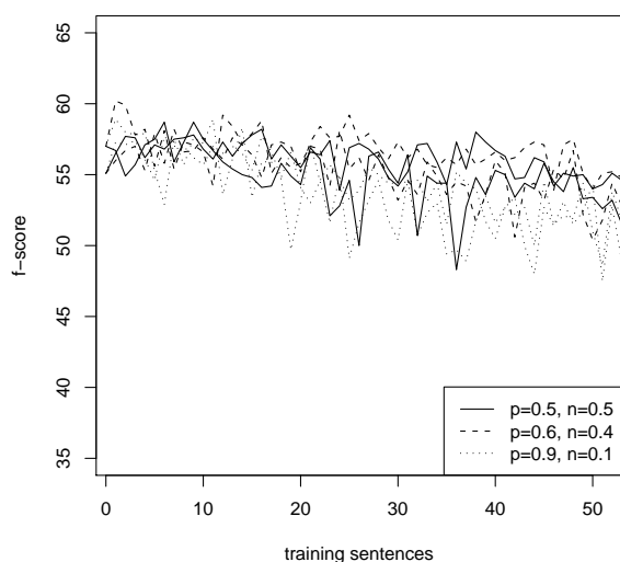
Figure 5: Co-training with selection bias.
