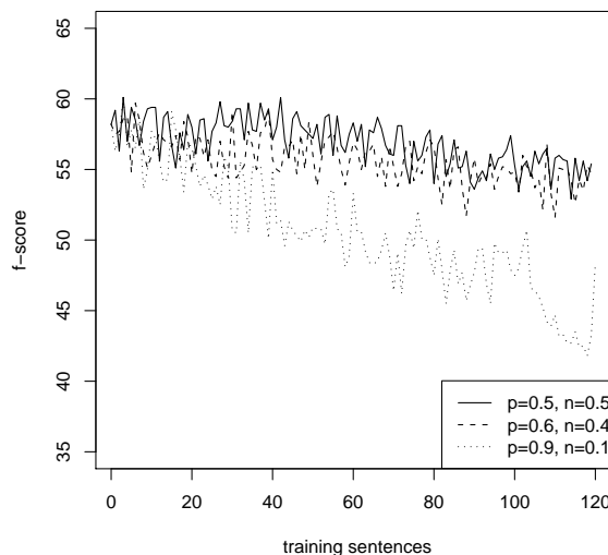
Figure 4: Self-training with selection bias.
