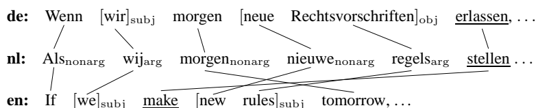
Figure 1: The argument (head) identification task.
