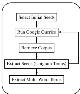
Figure 1: The BootCaT flow
