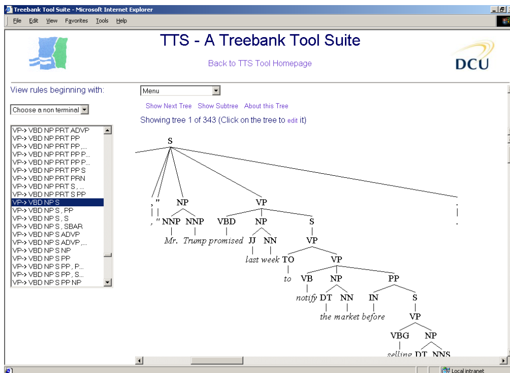
Figure 5. TTS limiting the rule VP→ VBD NP S
